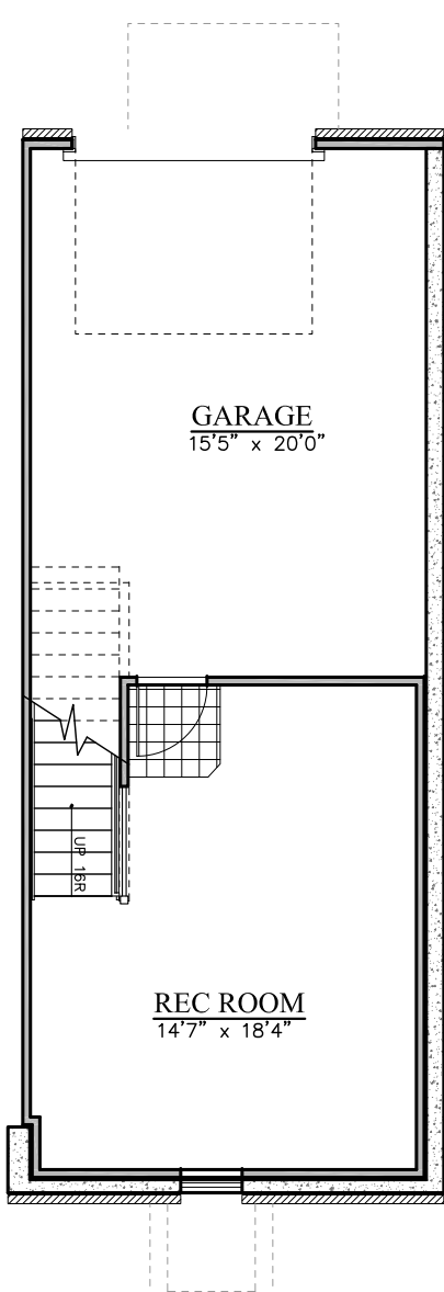
BASEMENT LEVEL
