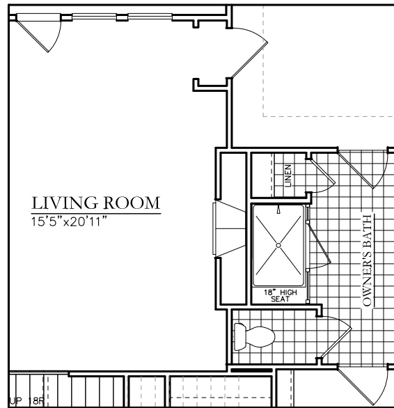
OPT. FIREPLACE
