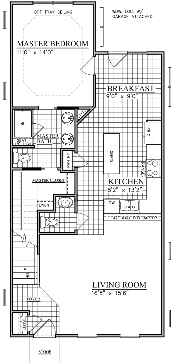
1ST FLOOR
