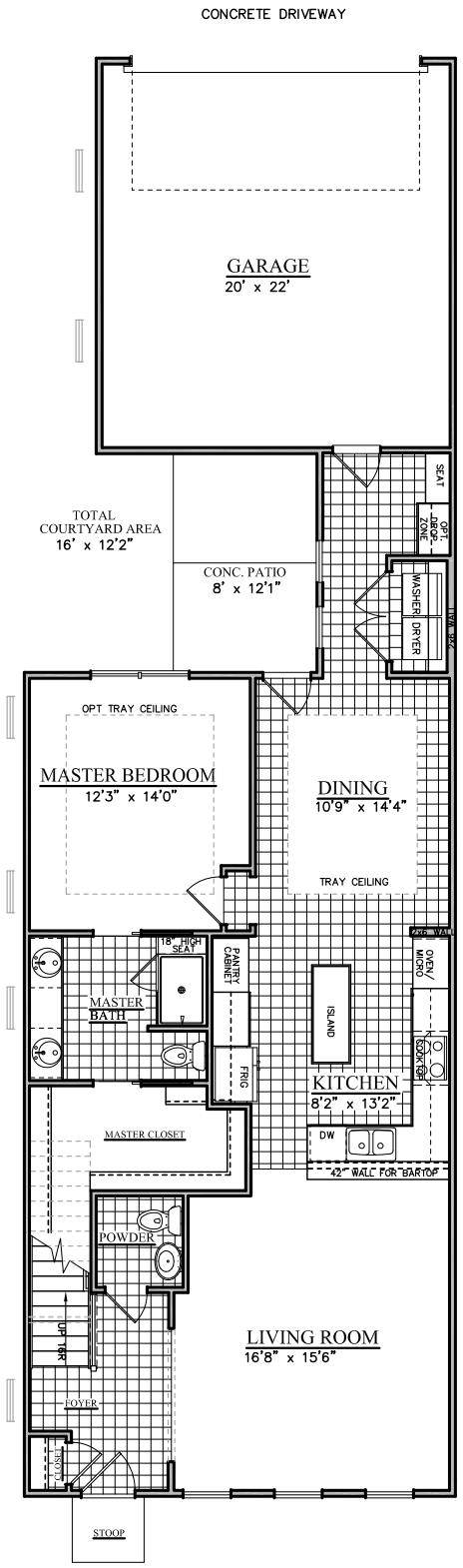
1ST FLOOR
