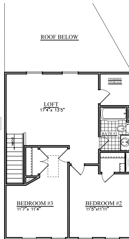
2ND FLOOR
